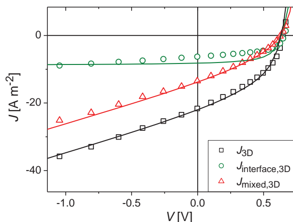
Figure 12. Simulated J - V curves for the total current and the two separate components calculated with the 3D (symbols) and with the parallel model (lines). This plot display Simulation 2.
